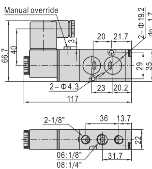
4M220(Terminal)
