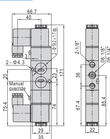
4M220(Terminal)
